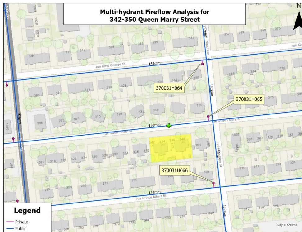
342-348 Queen Street: fire flow analysis, multi-hydrant locations
