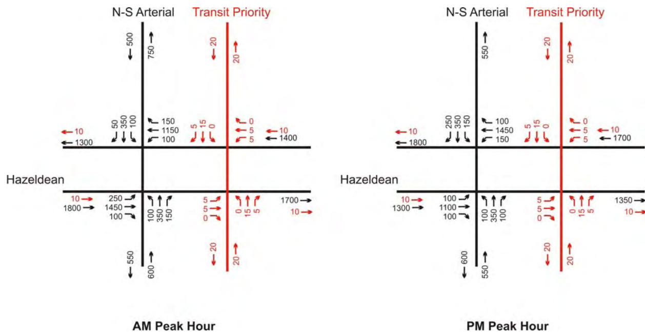
Figure 5: Projected Peak Hour Traffic Volumes: \pm 2023 : pcus/ buses
