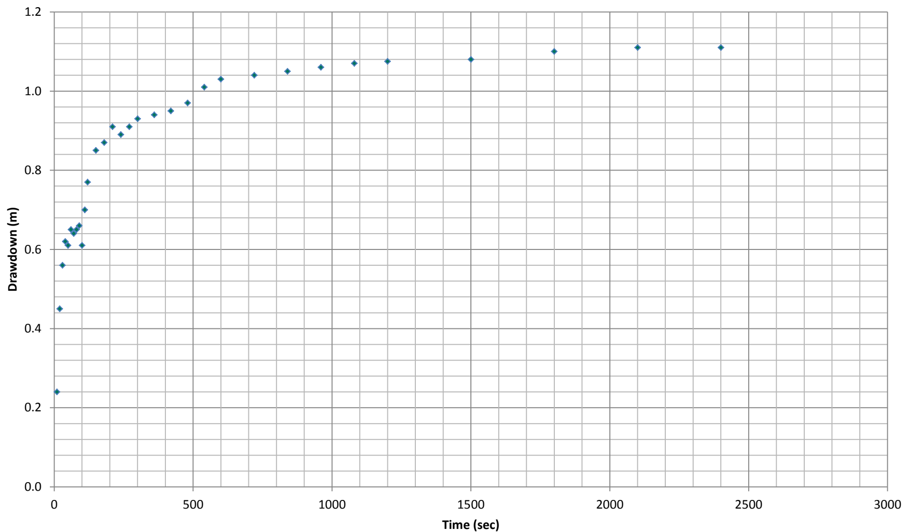
Time-Drawdown Relationship - March 14, 2013
