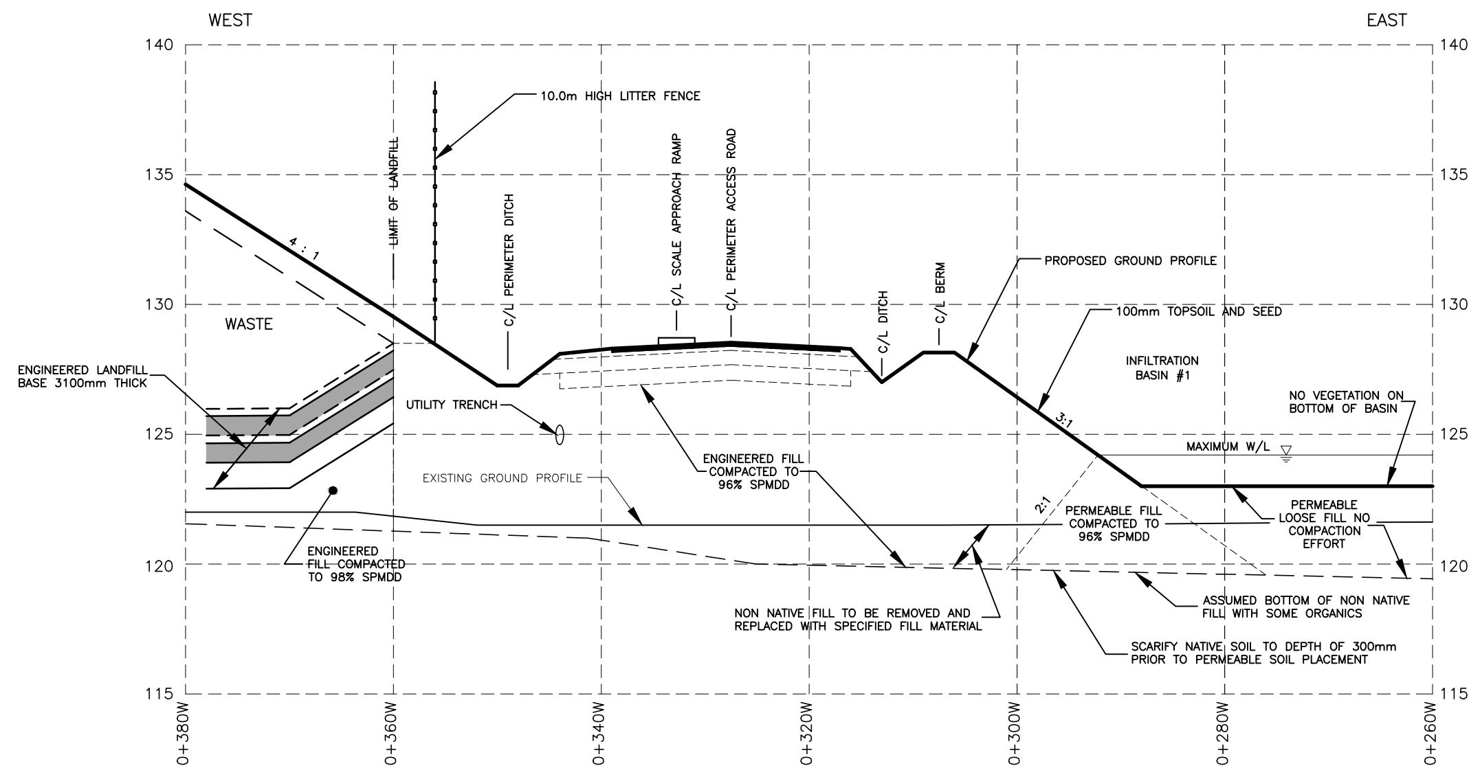
SECTION F GRID LINE 1+000W SCALES 1 : 500 HORIZONTAL 1 : 200 VERTICAL
