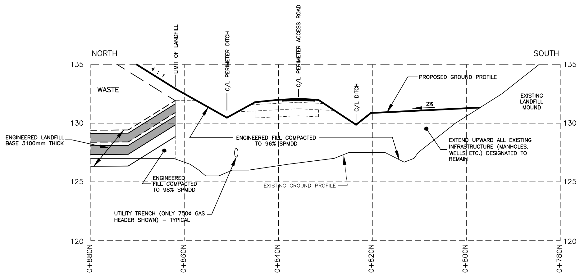
SECTION H GRID LINE 1+000W SCALES 1 : 500 HORIZONTAL 1 : 200 VERTICAL
