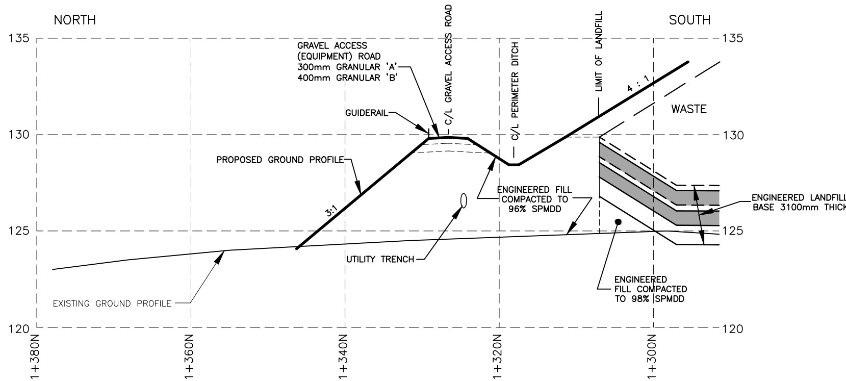
SECTION J GRID LINE 1+100W SCALES 1 : 500 HORIZONTAL 1 : 200 VERTICAL
