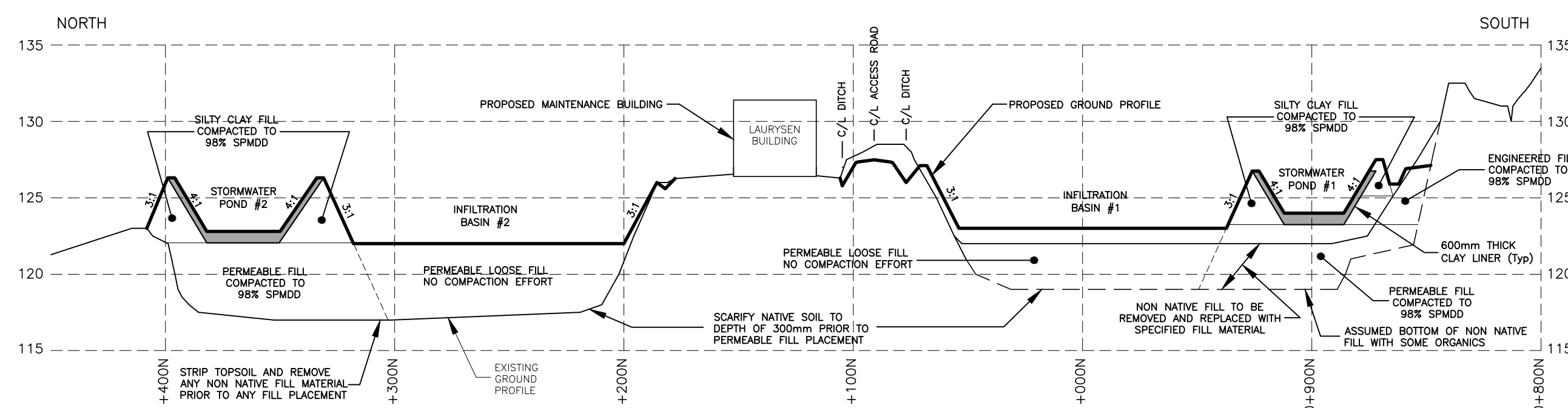
SECTION K GRID LINE 0+200W SCALES 1 : 2000 HORIZONTAL 1 : 300 VERTICAL
