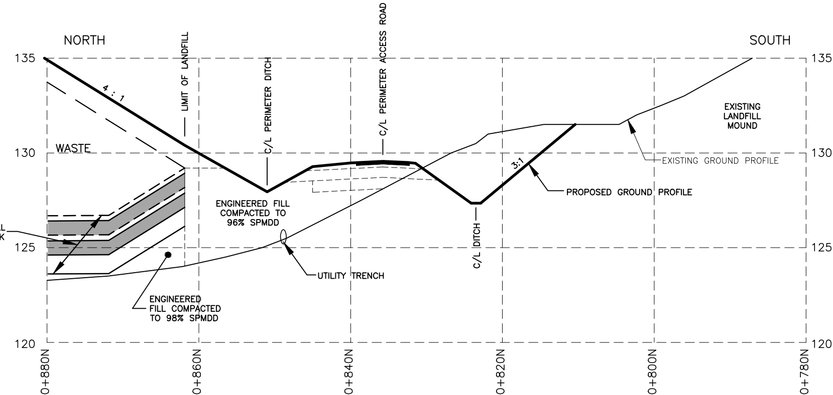
SECTION G GRID LINE 0+400W SCALES 1 : 500 HORIZONTAL 1 : 200 VERTICAL
