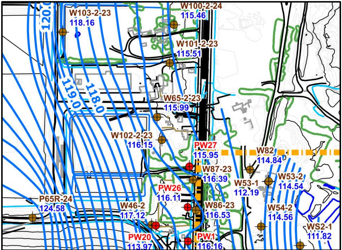
Figure 2 – Interpreted groundwater flow in the overburden in the vicinity of the Laurysen Building Well (adapted from Figure 7 of 2024 Annual Report Waste Management of Canada West Carleton Environmental Centre Ottawa, Ontario. Prepared for Waste Management of Canada Corporation. Prepared by BluMetric Environmental Inc. dated March 31, 2025
