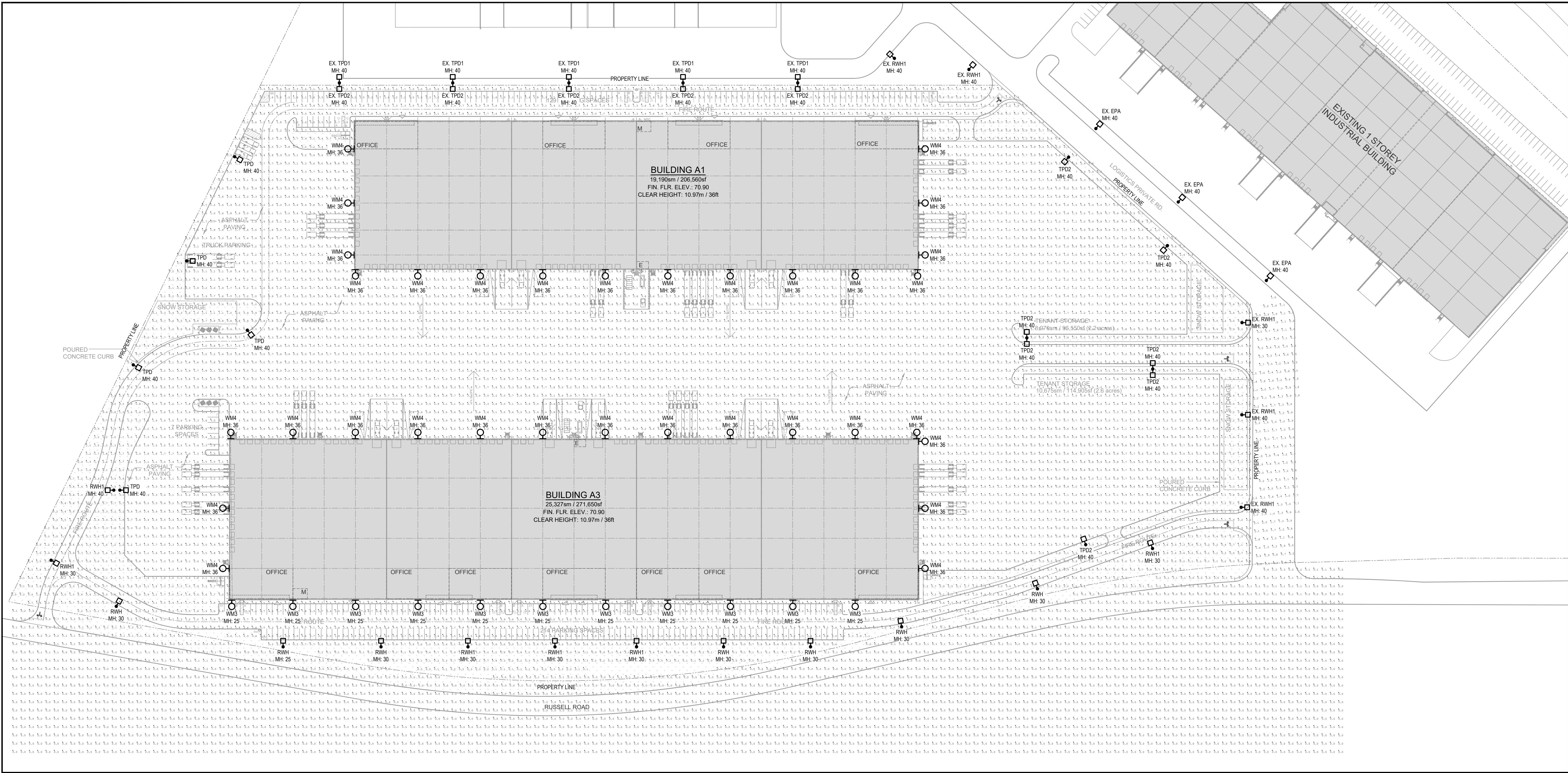
1 SITE PLAN - PHOTOMETRIC SCALE: 1 : 1000
