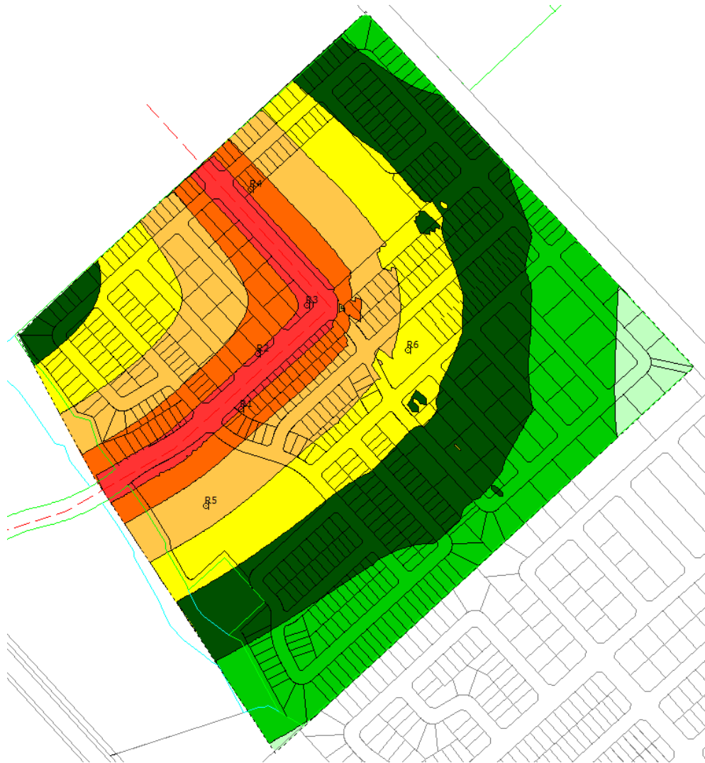
FIGURE 5: GROUND LEVEL NOISE CONTOURS FOR THE SITE (DAYTIME PERIOD)
