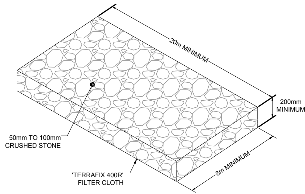
MUD MAT DETAIL NTS
