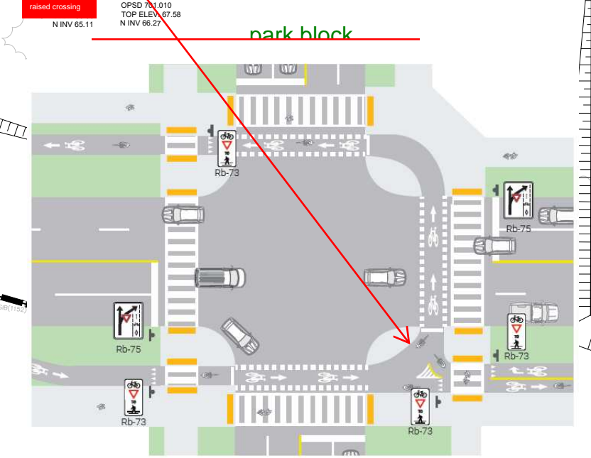
Figure 6.87 - One-way / Two-way Transition at Intersection
