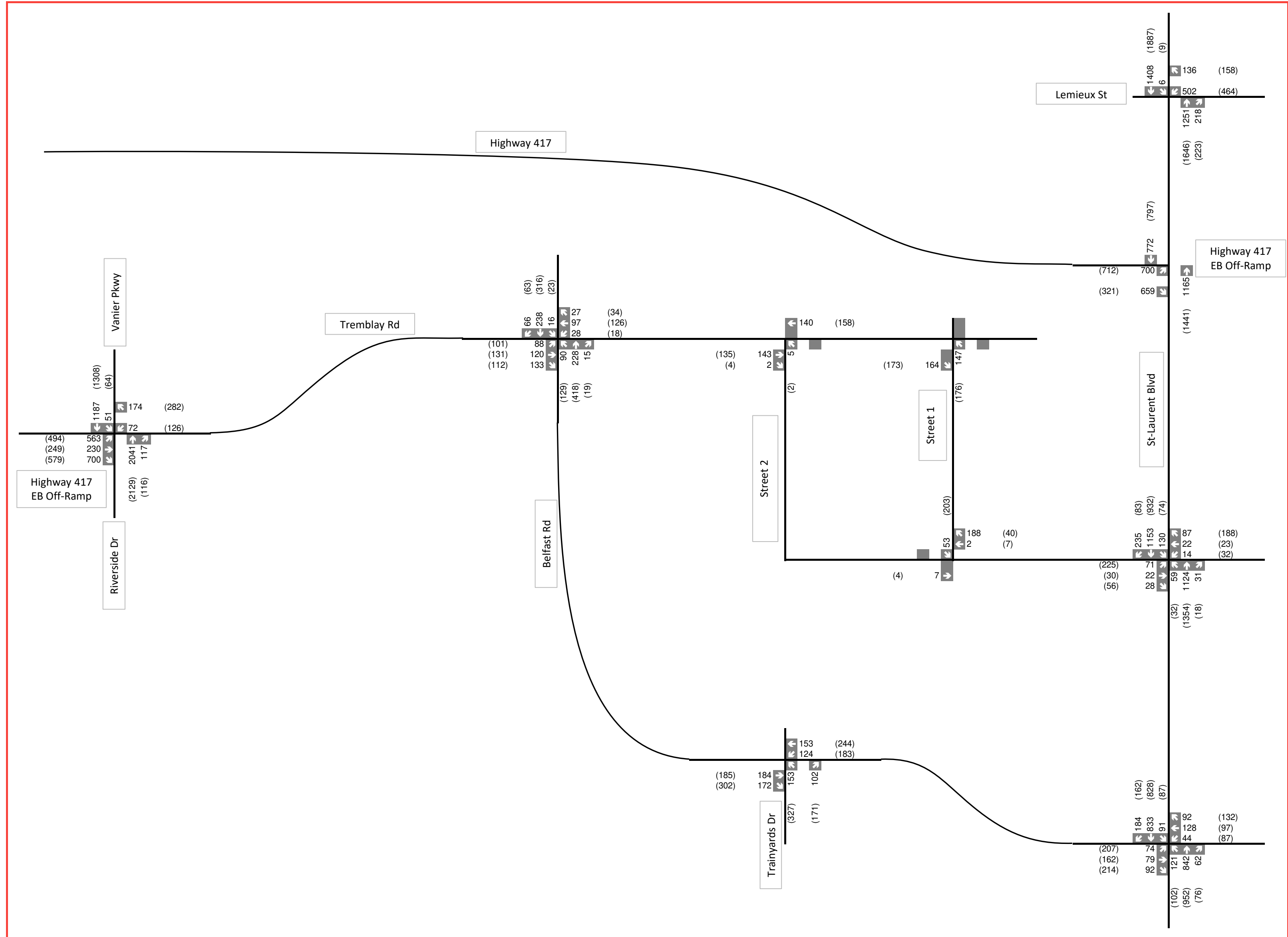
Figure 3-12 2029 Total Traffic
