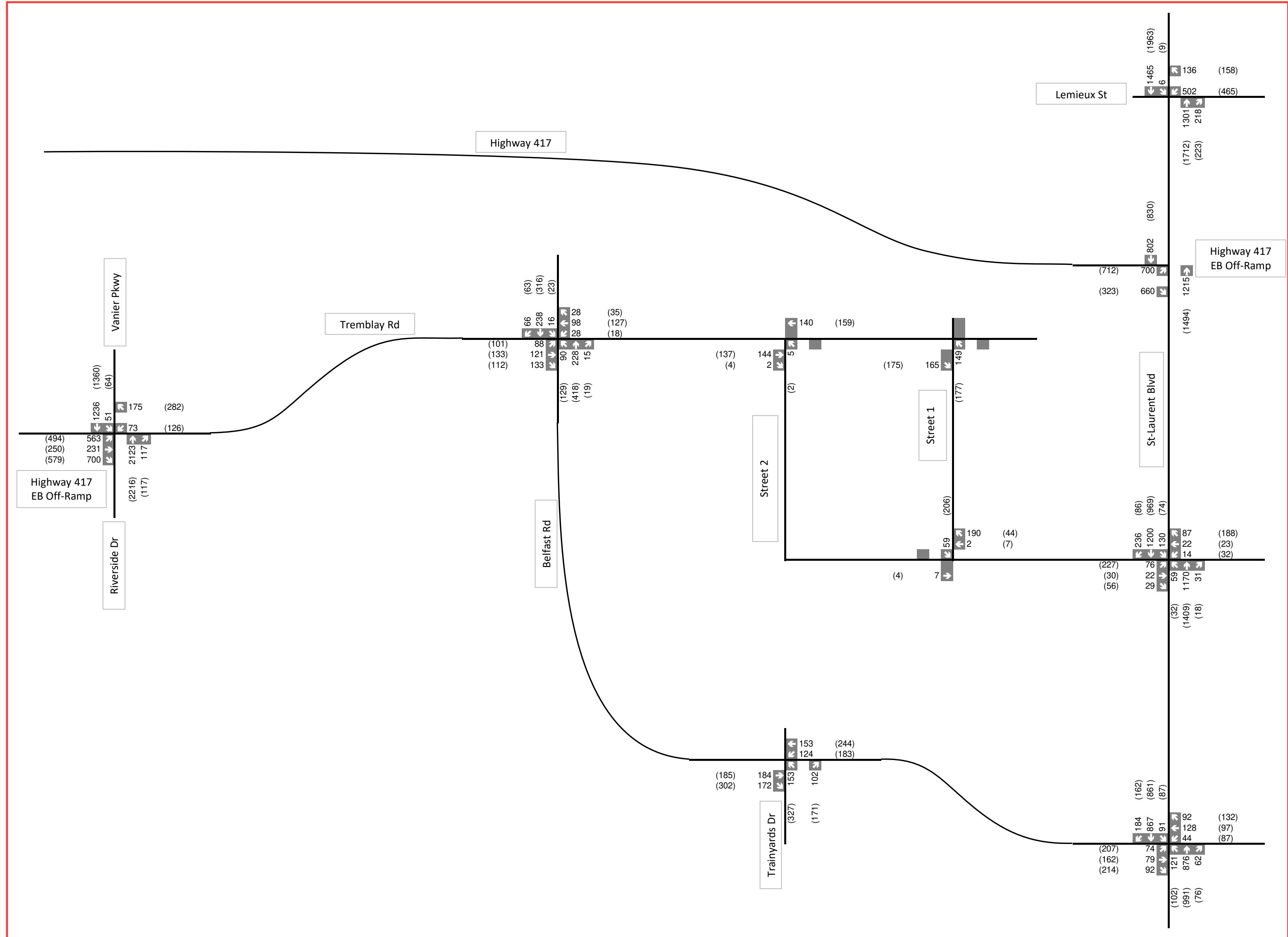
Figure 3-13 2033 Total Traffic
