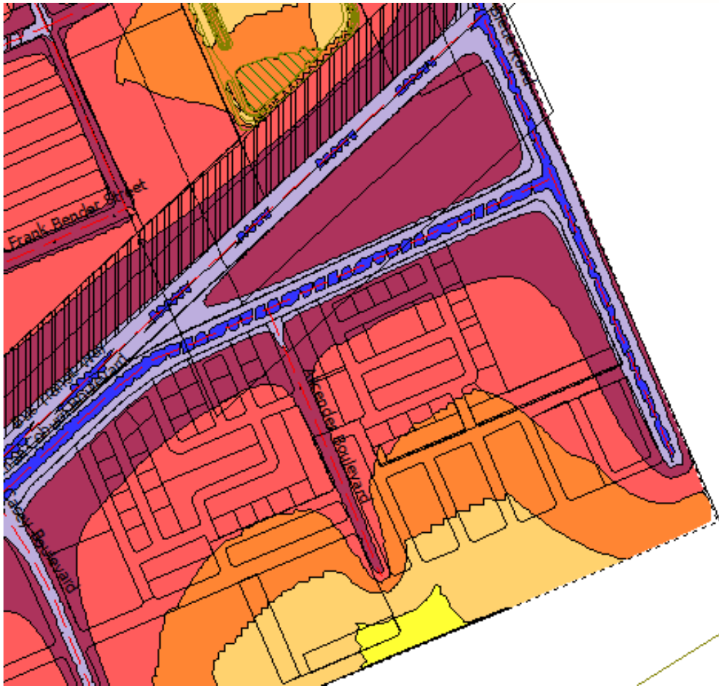
FIGURE 5: DAYTIME TRAFFIC NOISE CONTOURS (1.5 M ABOVE GRADE)
