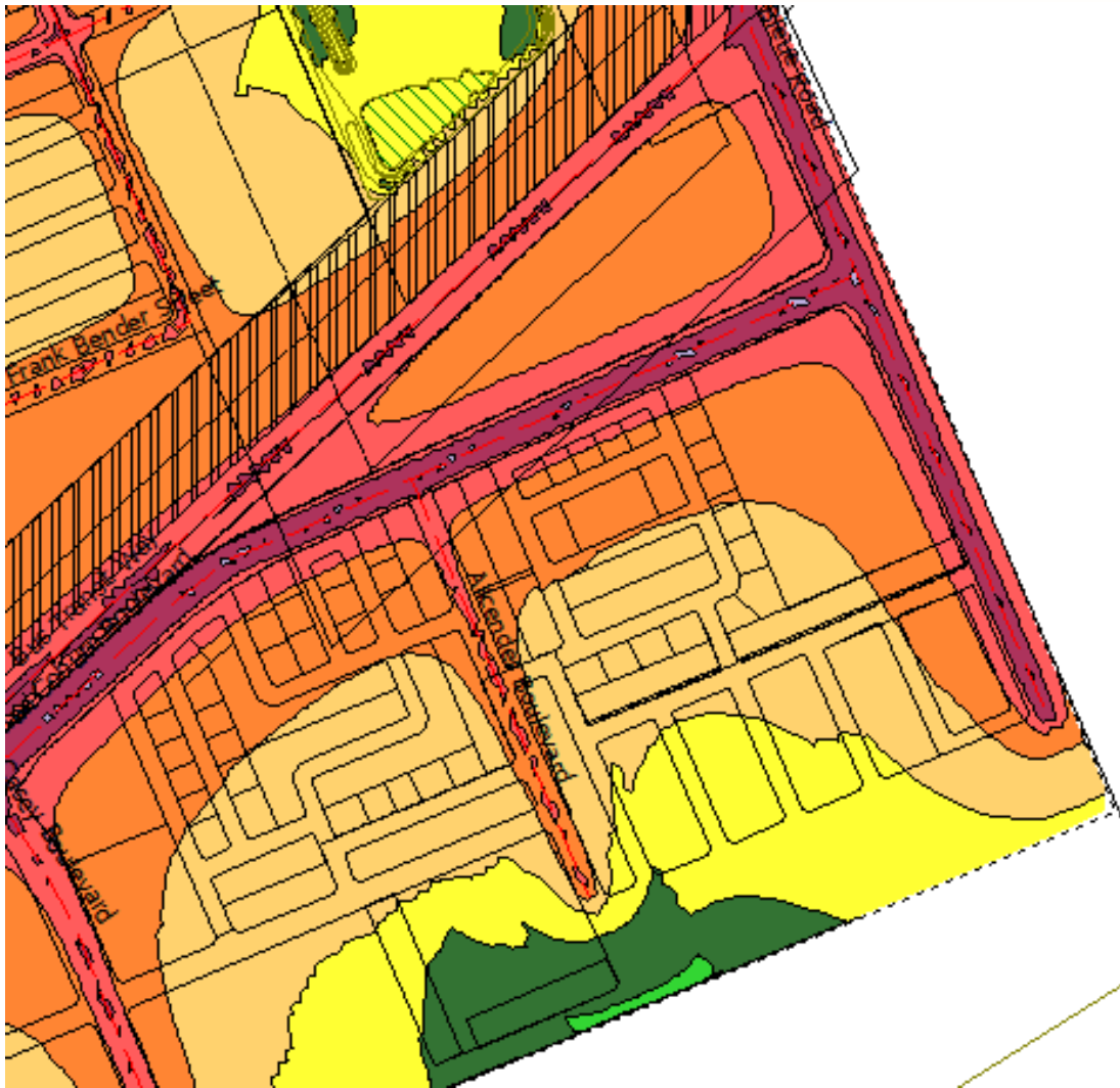
FIGURE 6: NIGHTTIME TRAFFIC NOISE CONTOURS (1.5 M ABOVE GRADE)
