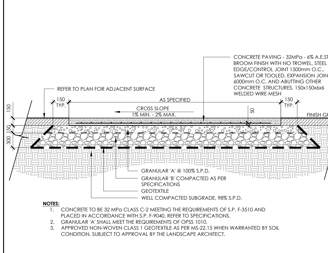
5 HEAVY DUTY CONCRETE PAVING N.T.S.
