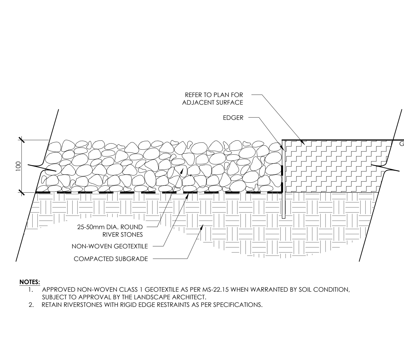
10 RIVER STONE PAVING N.T.S.
