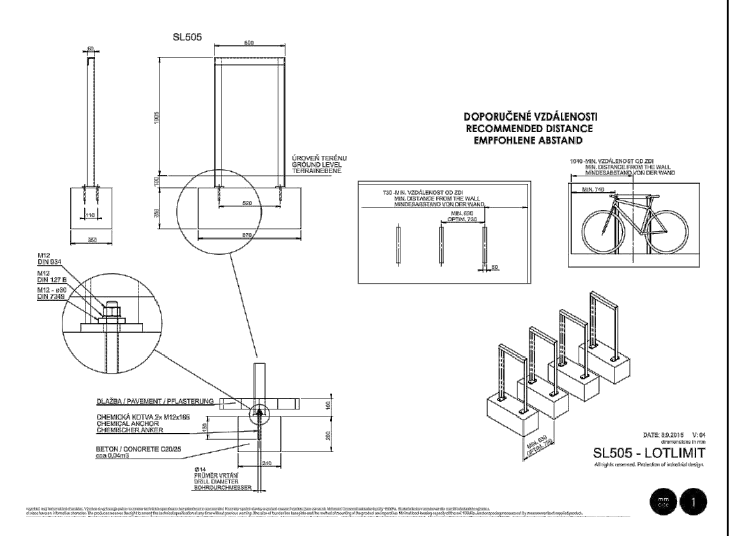
8 BIKE RACK - ON CIP CONCRETE N.T.S.
