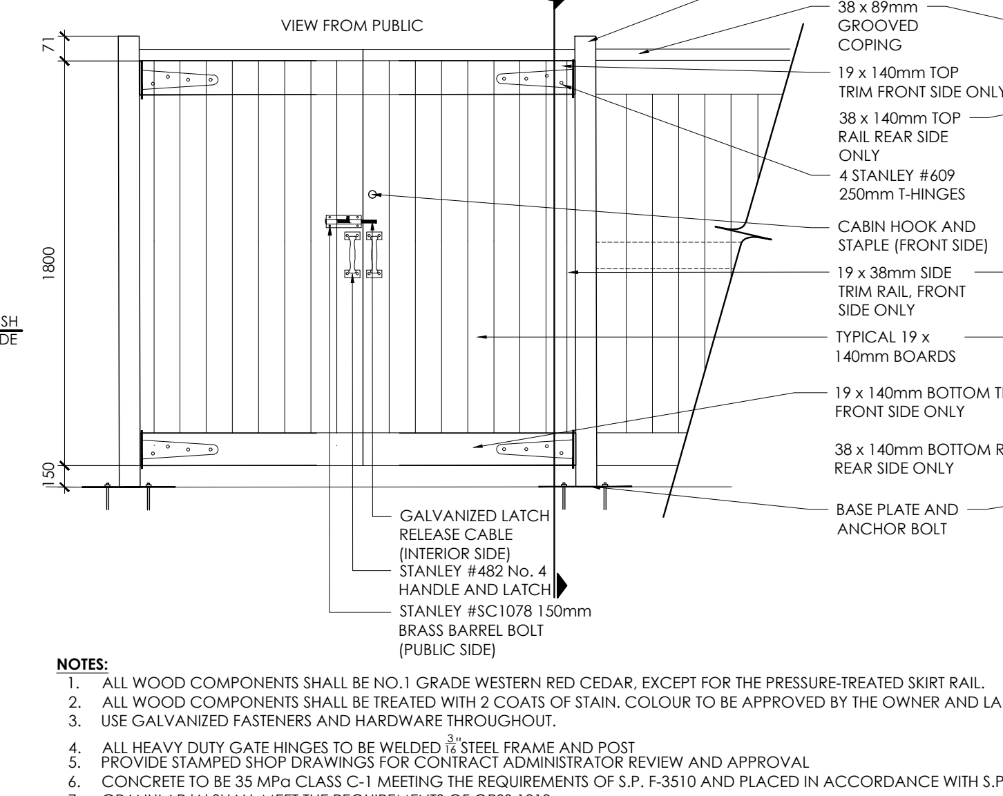
11 2.0m HT. PEDESTRIAN ACCESS GATE AND FENCE N.T.S.
