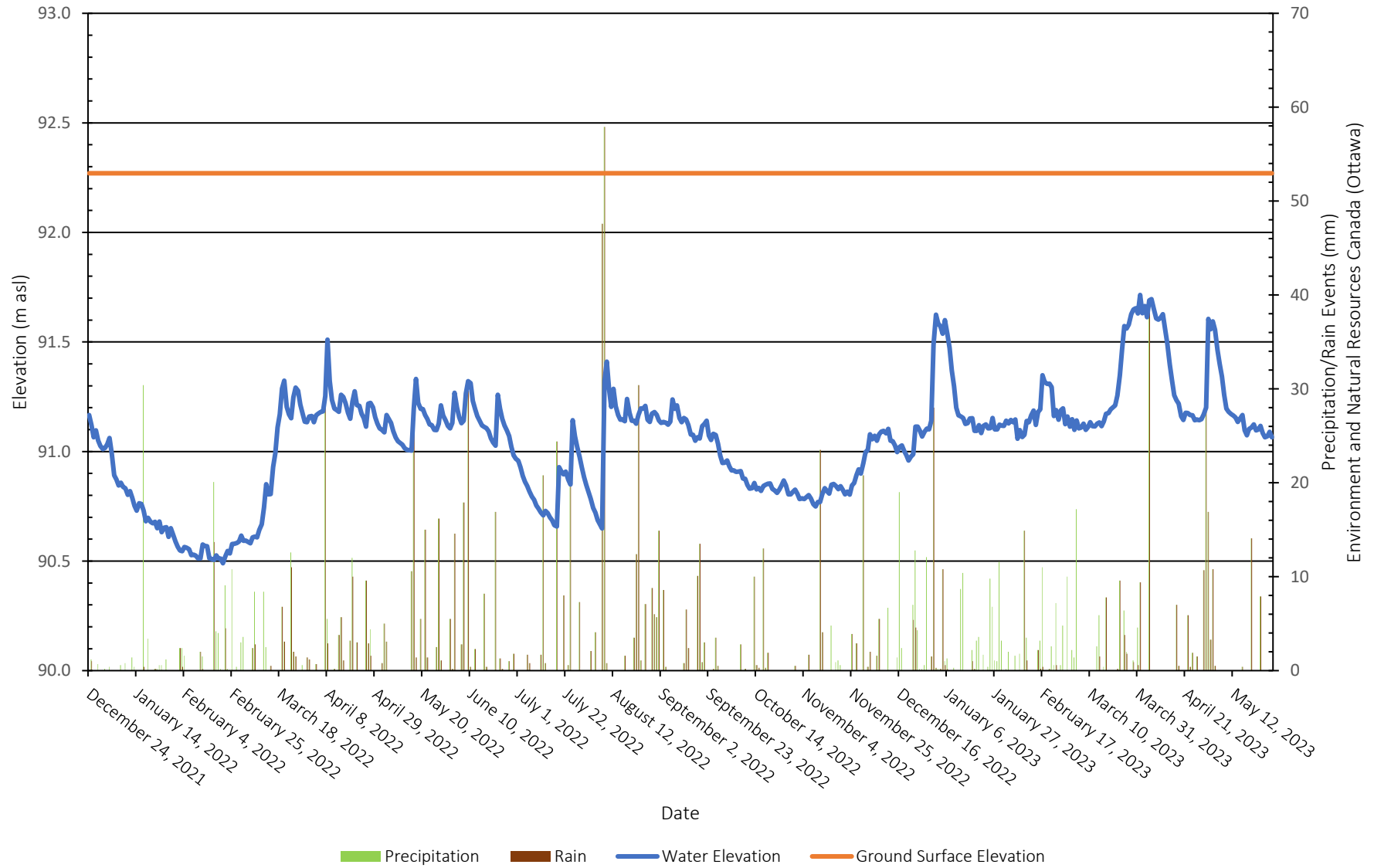
Figure 7: BH6-21 - Monitoring Well Water Elevations
