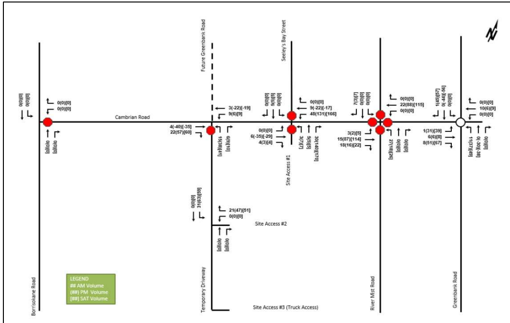
Figure 24: 3831 Cambrian Road Site Generated Traffic Volumes
