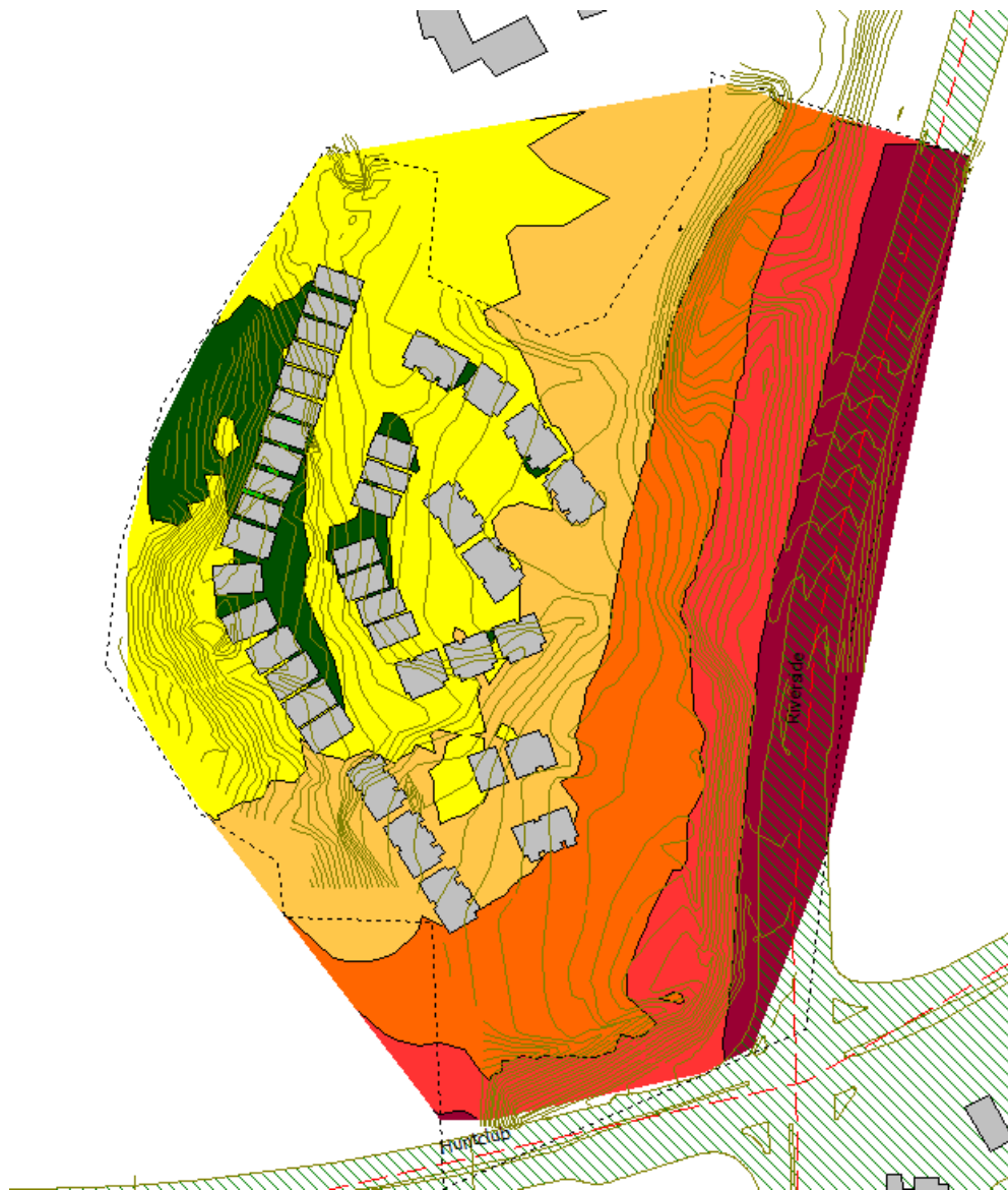
FIGURE 4: NIGHTTIME TRAFFIC NOISE CONTOURS, LOW-RISE ONLY (4.5 M ABOVE GRADE)
