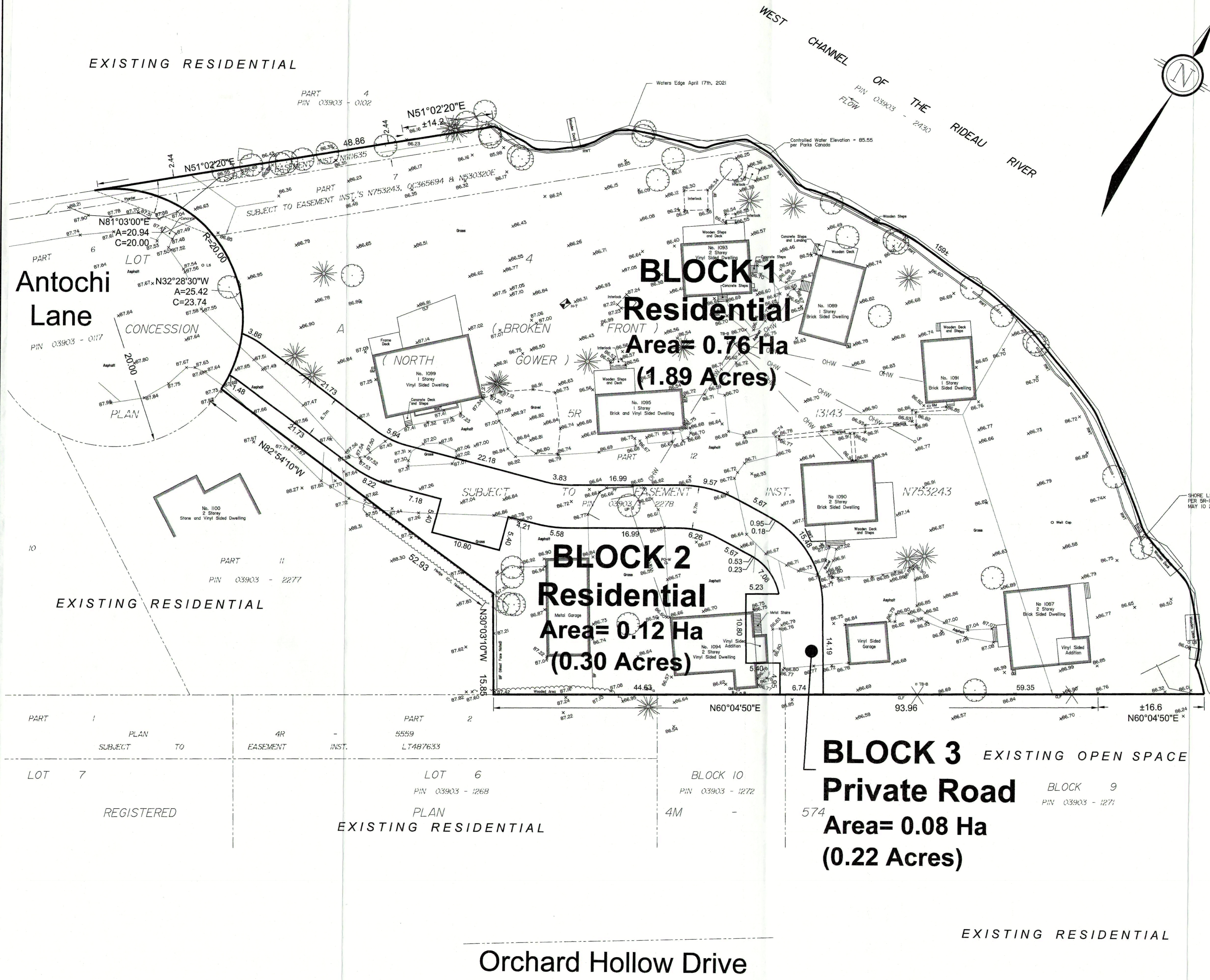
KEY MAP NOT TO SCALE METRIC : MEASUREMENTS SHOWN ON THIS PLAN ARE IN METRES AND CAN BE CONVERTED TO FEET BY DIVIDING BY 0.3048.
