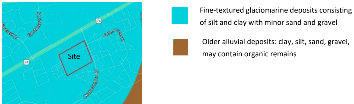
Image 1 – Surficial Geology
