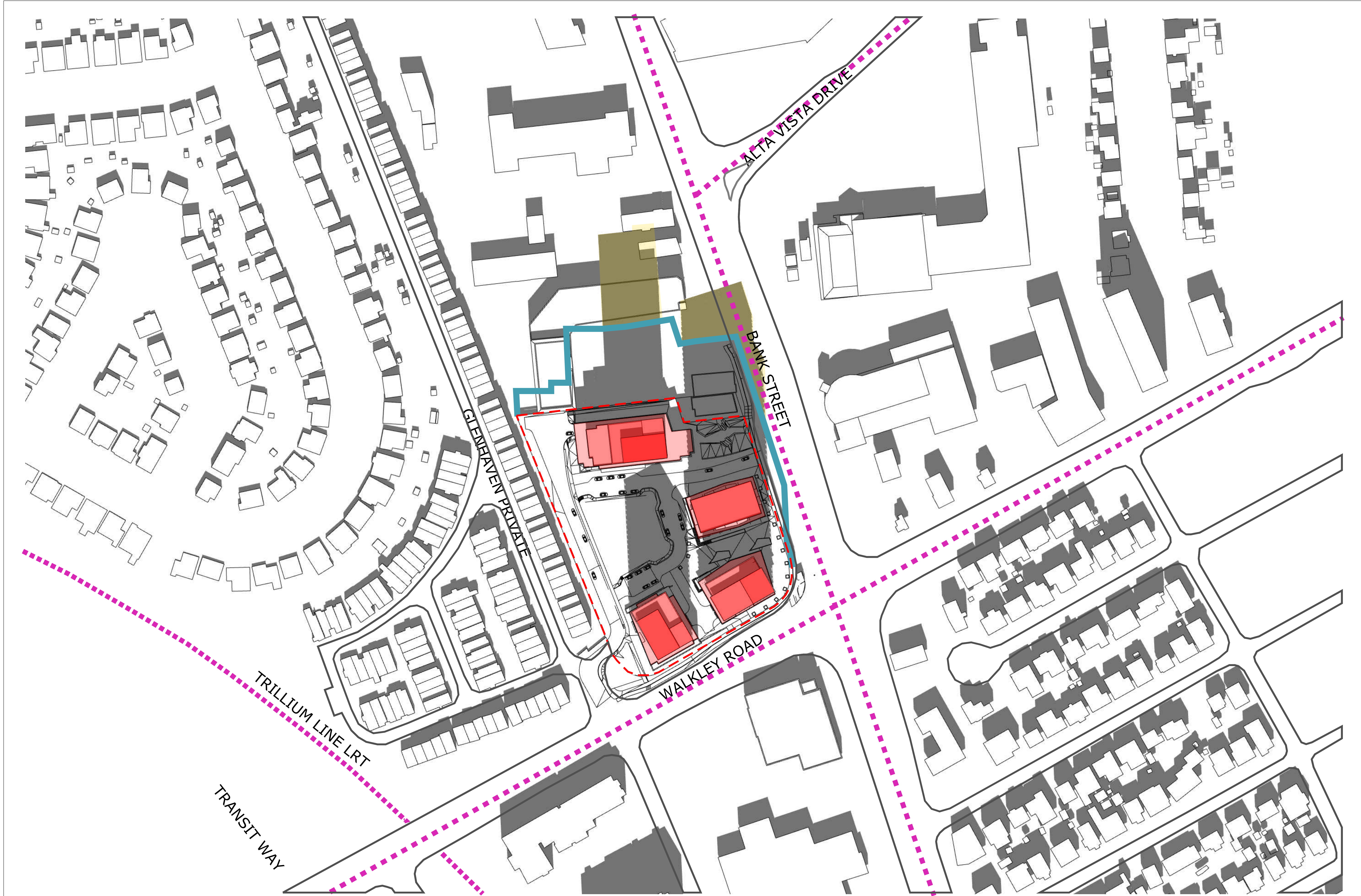
TOP-VIEW SHADOW ANALYSIS MARCH 1:00pm APPLICATION NO.: D00-00-00-0000
